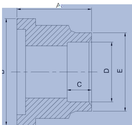
Casing
